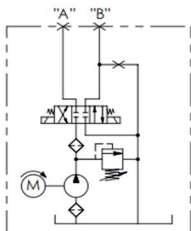
HYDRAULIC CIRCUIT 114C
