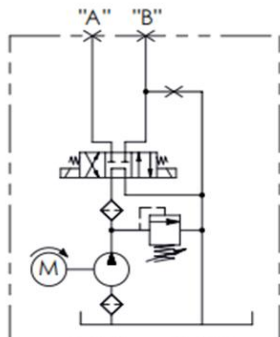
HYDRAULIC CIRCUIT 114B
